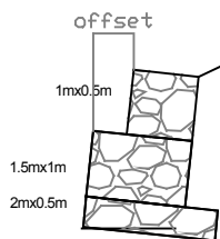
Volume =3.5cum/m run
