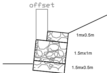
Volume =2.75cum/m run
