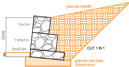
Volume =3.5cum/m run
