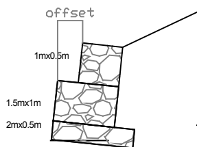
Volume =3.5cum/m run
