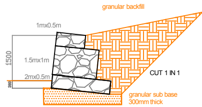
Volume =3.0cum/m run
