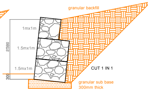
Volume =4cum/m run
