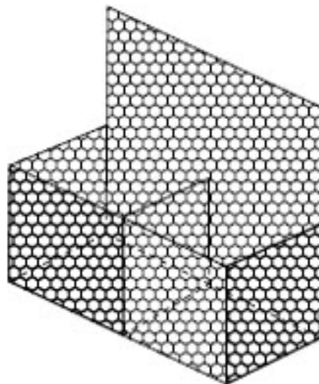
GABION FORMED INTO BOX SHAPE ON SITE
